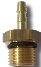
CODE AEBRC002 ASSEMBLED G 1/4 HOSE CONNECTION D.4
